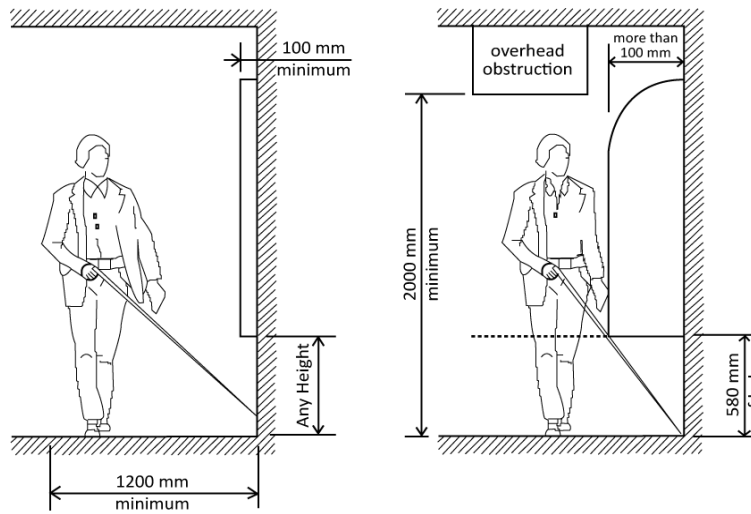
Figure 3.D.4 Limit of protruding objects
