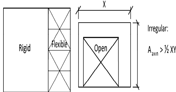
(c) Diaphragm discontinuity
