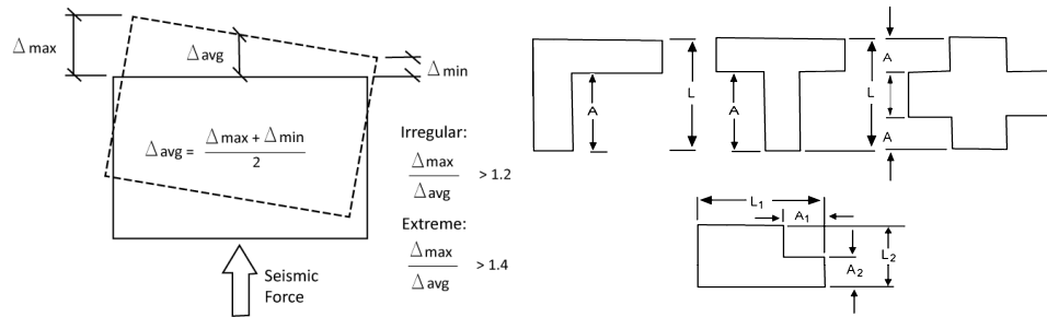
(a) Torsional Irregularity
