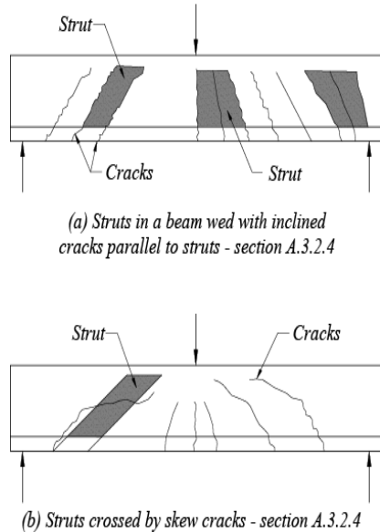
Figure 6.I.10 Types of struts
